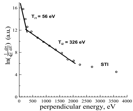
Fig. 3. Charge exchange neutral (CXN) energy spectrum corresponds to two-temperature ion energy distribution + suprathermal tail.
