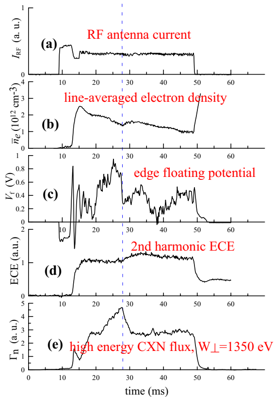
Fig. 4. Some indications of H-mode transition. The start of transition is indicated by a vertical dashed line.
