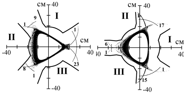
Fig. 2. Disposition of divertor electric probe arrays in the spacings between the helical coils in the poloidal cross-sections A7 (left) and D7 (right)
