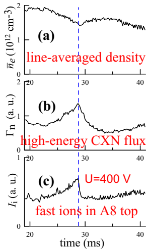
Fig. 6. Time evolution of density \bar{n}_e (a), high energy charge exchange neutral (CXN) flux, \Gamma_n (b) and fast ion flow out flowing to DPF, I_i (c) in the vicinity of H-transition in A8 top.
