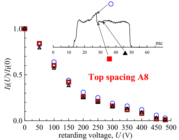
Fig. 7. Normalized ion current I_i(U)/I_i(0) to the collector of IEA versus retarding voltage U in the top spacing A8.
