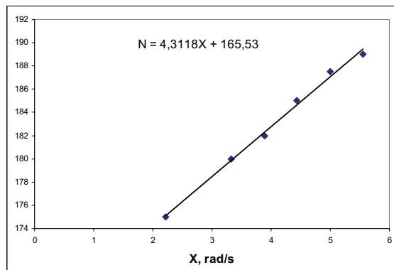
Fig. 2. Dependence of the resonant transmission of the rotation angle of the rotor for frequency of rotation 50 Hz
